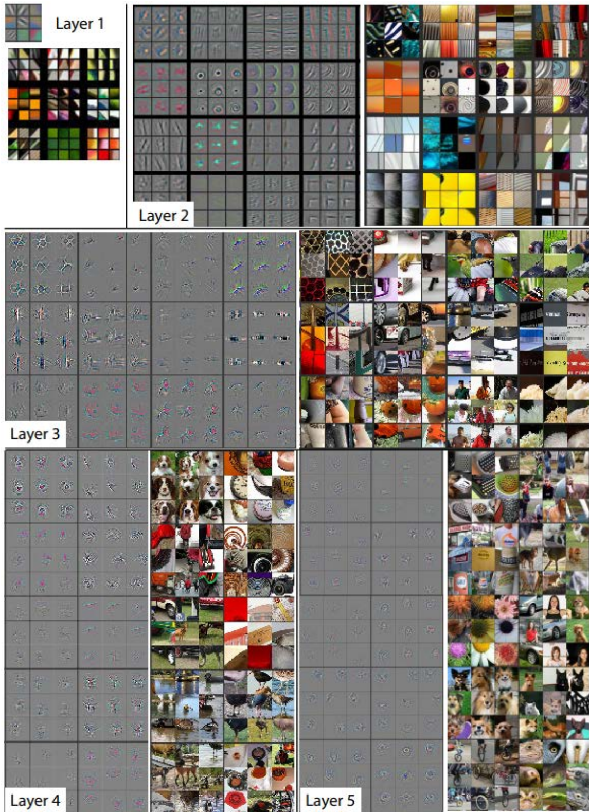
Figure 10. Features extracted by a deep convolutional neural network [17]
